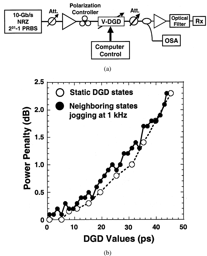
Fig. 8. System evaluation of the tunable DGD module. (a) Experimental setup of a 10-Gb/s NRZ ( 2^{31} - 1 PRBS) link. (b) Measured power penalties for two cases. Open circle: the DGD module remains static after changing state. Solid circle: the DGD module keeps jogging back and forth between neighboring states at 1 kHz.
