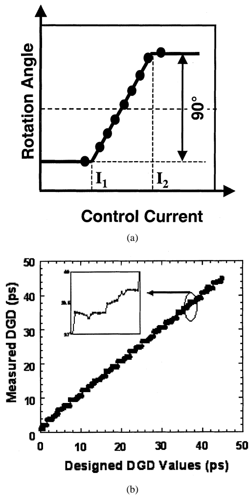
Fig. 7. Characterization of transient DGD effects during polarization switching. (a) Quasi-static measurement of transient DGD by step-varying the control current of the MO switches. (b) Measurement of transient DGD by equivalent small polarization variation between different DGD values from 0 to 45 ps.
