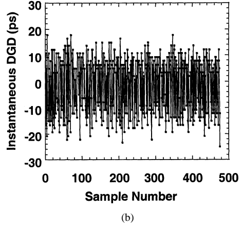
Fig. 6. Repeatable DGD generation is used to generate dynamic first-order PMD distribution with tunable average values. (a) First-order PMD distribution of 500 samples with an average DGD of 10 ps. (b) Instantaneous DGD values of the samples.
