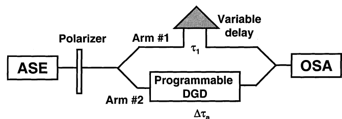
Fig. 4. TTD measurement setup using an ASE broad-band source. OSA: Optical spectrum analyzer.
