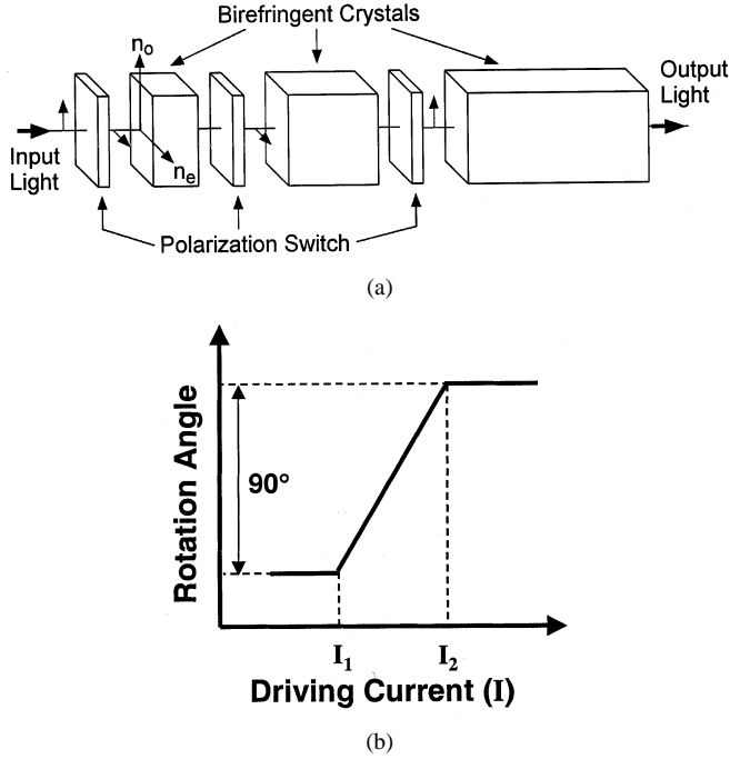
Fig. 1. (a) Illustration of a programmable DGD module based on polarization switching. (b) Typical response curve of a magneto-optic (MO) polarization switch.
