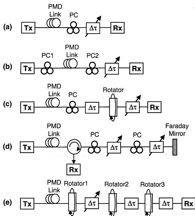
Fig. 9. Different approaches for PMD compensation using variable DGD modules. (a) [9]. (b) [10]. (c) [11]. (d) [12]. [13]. (e) [14].
