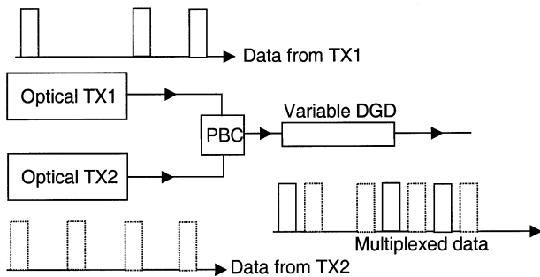
Fig. 11. Illustration of data bit alignment using the delay module described in this paper.
