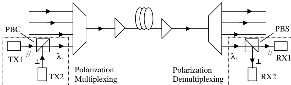
Fig. 1. Illustration of a polarization division multiplexing (PDM) system
