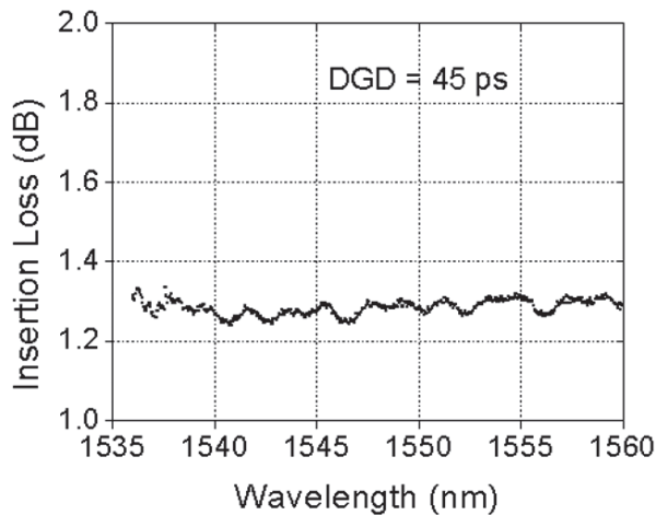
Figure DGD-2. Insertion loss vs. wavelength.
