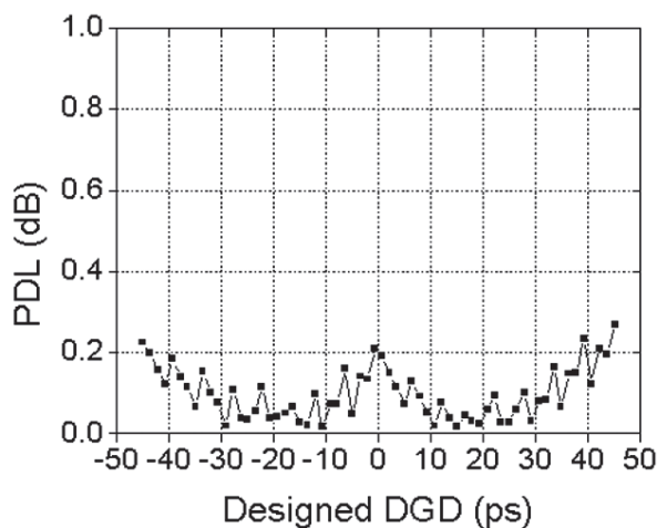
Figure DGD-3. PDL vs. DGD setting
