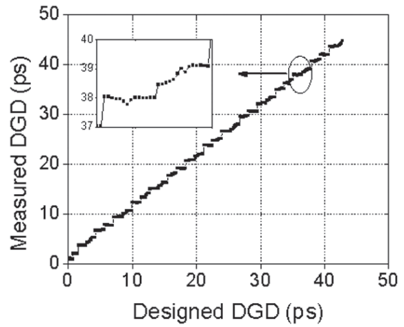
Figure DGD-4. Detailed DGD switching process and transient DGD value measurement results.
