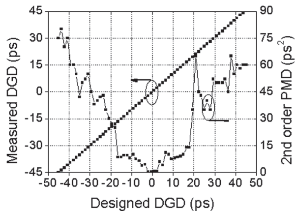
Figure DGD-1. Measured DGD and 2nd order PMD vs. set DGD.
