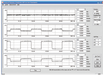
Fig. 2 Oscilloscope display of 4 Stokes parameters, with square wave polarization modulation
