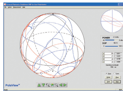
Fig. 1 Poincaré Sphere display of a polarization-scrambled input signal.
