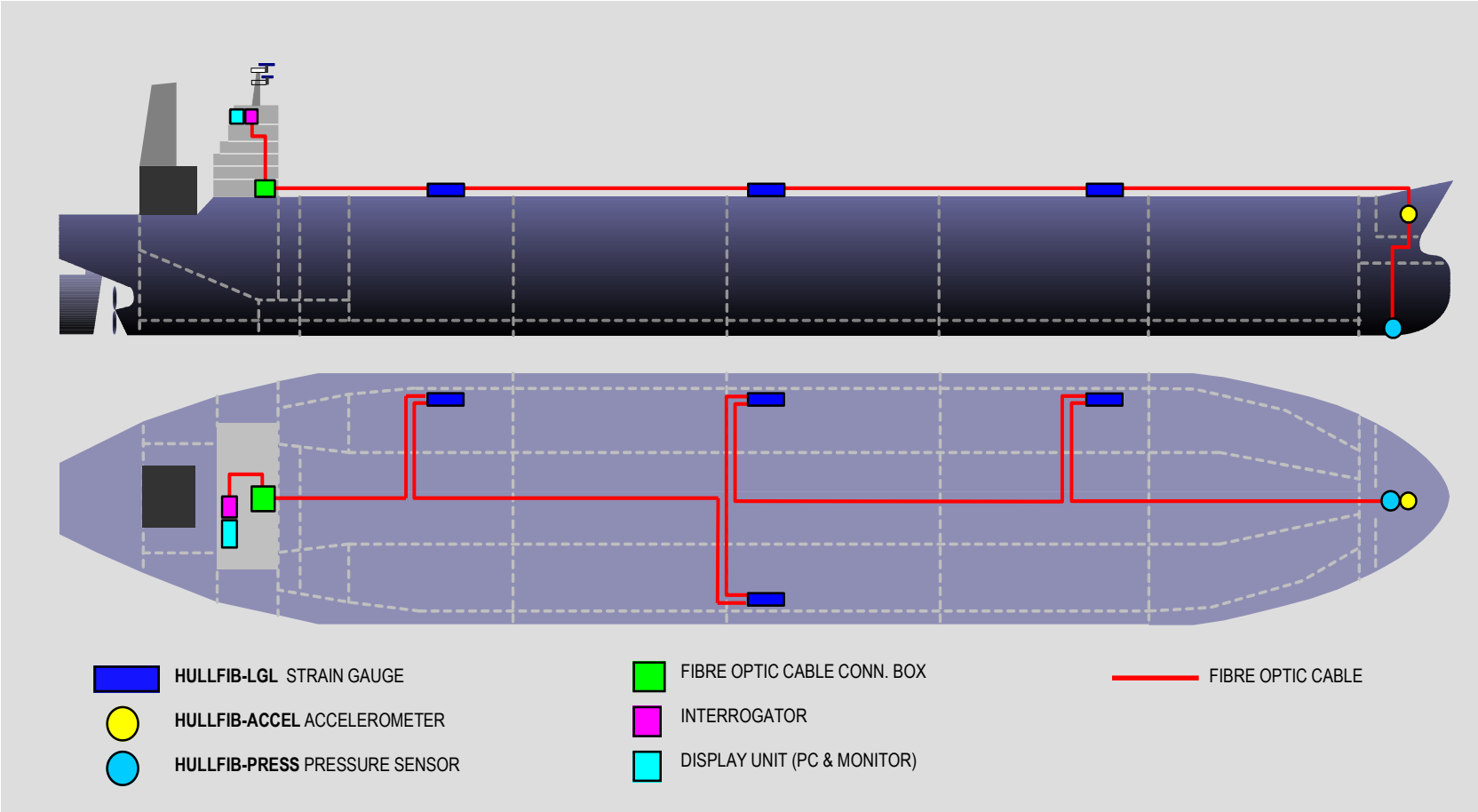
TYPICAL ARRANGEMENT OF HULLFIB
